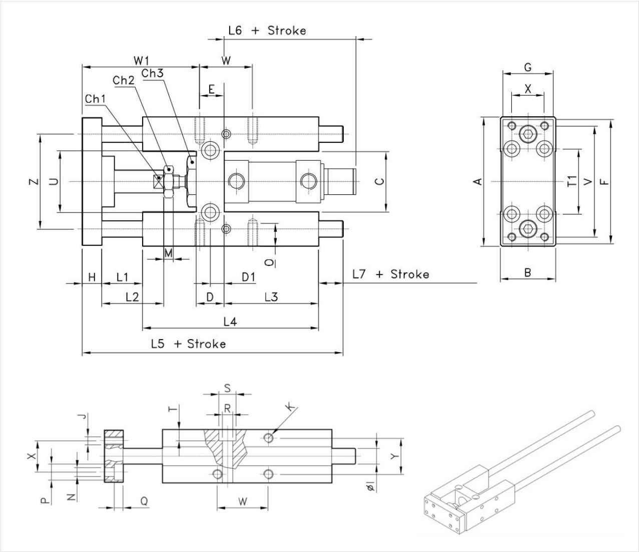
GUIDING UNIT H type Drawing for ISO 6432 cylinders
