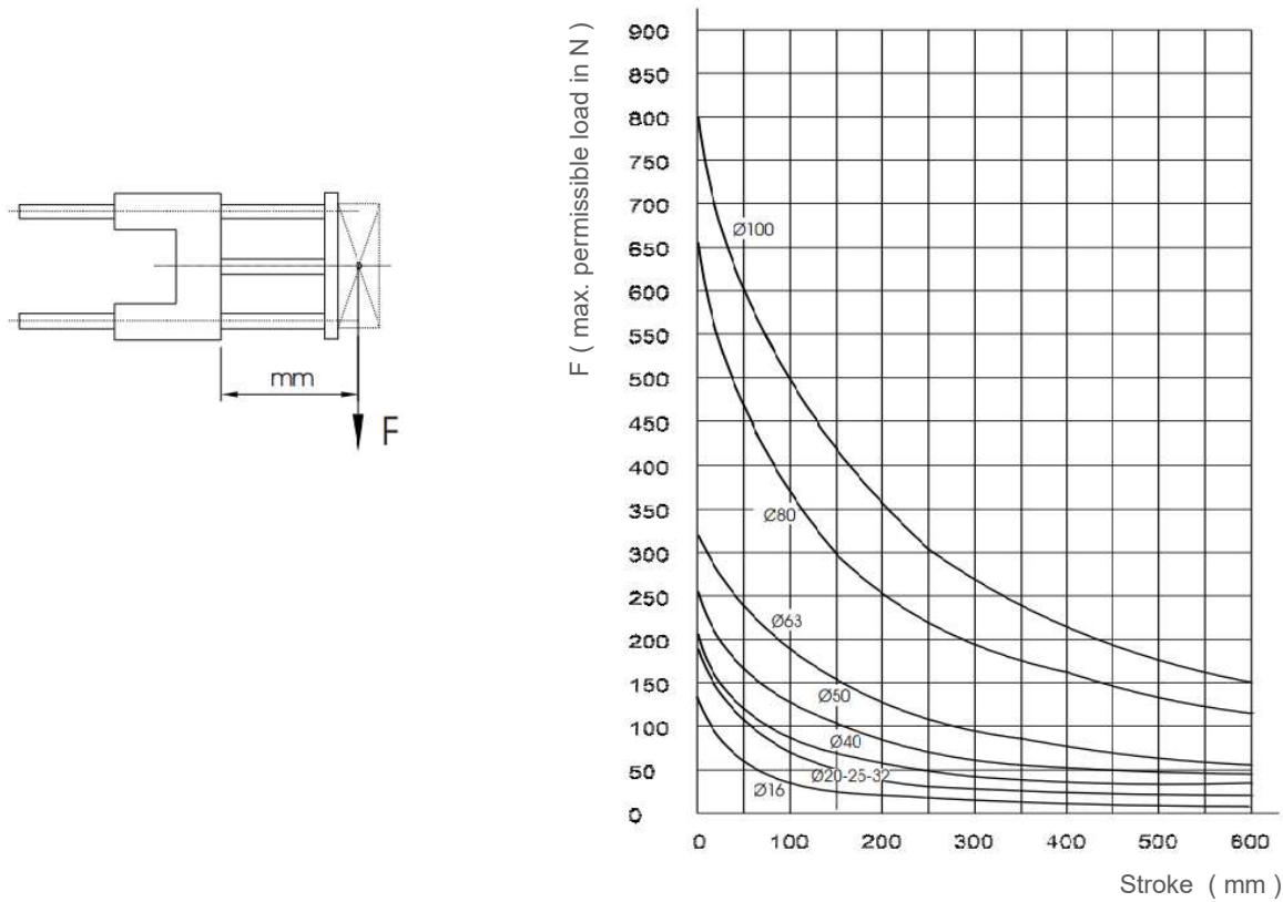
GUIDING UNIT Load – stroke graph . for U type
