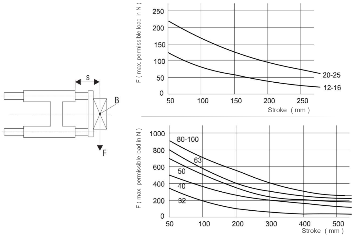
GUIDING UNIT Load – stroke graph . for H type
