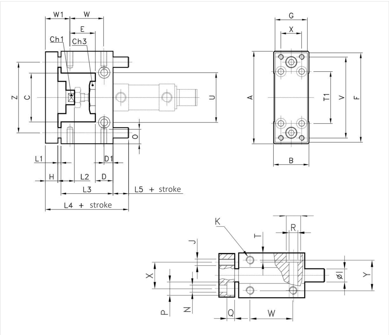
GUIDING UNIT U type Drawing for ISO 6432
