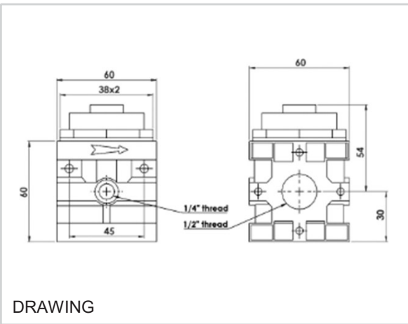
1/2" pilot REGULATOR
