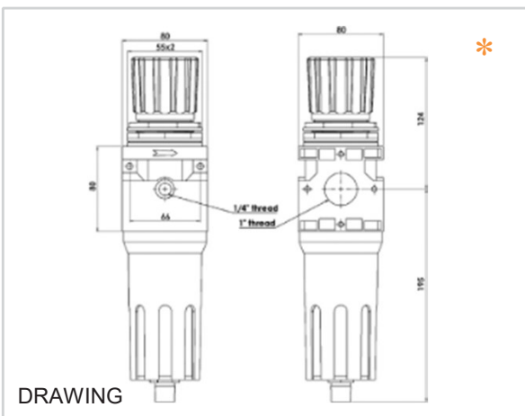
1" FILTER REGULATOR
