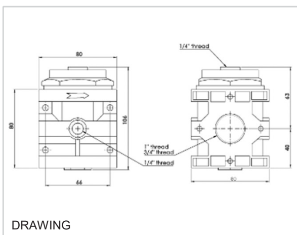
1" PILOT REGULATOR
