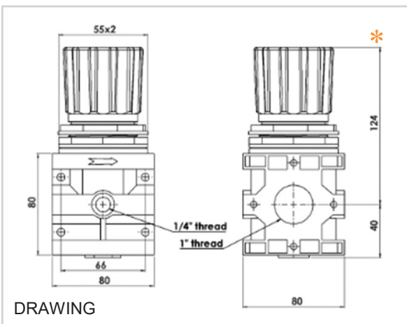
1" REGULATOR
