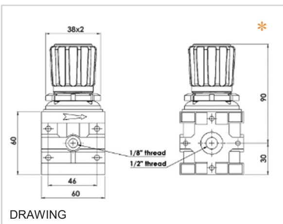
1/2 " REGULATOR
