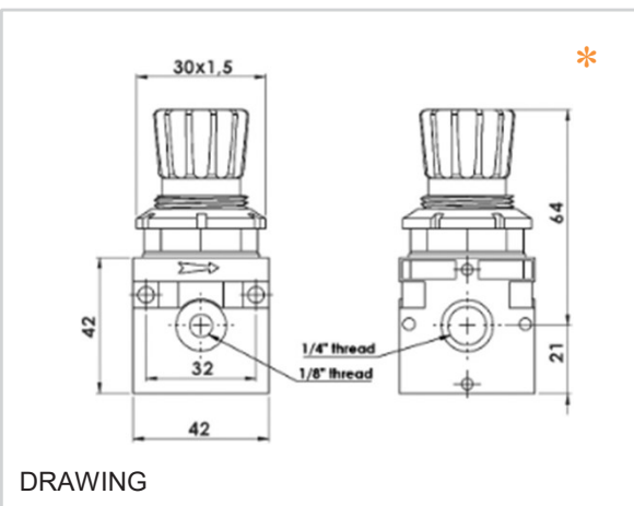
1/4 " REGULATOR
