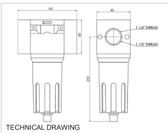
1 1/4" – 1 1/2" SMY FILTER
